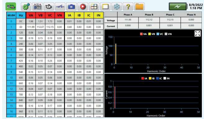
Figure 5: Harmonics table and graphic screen
